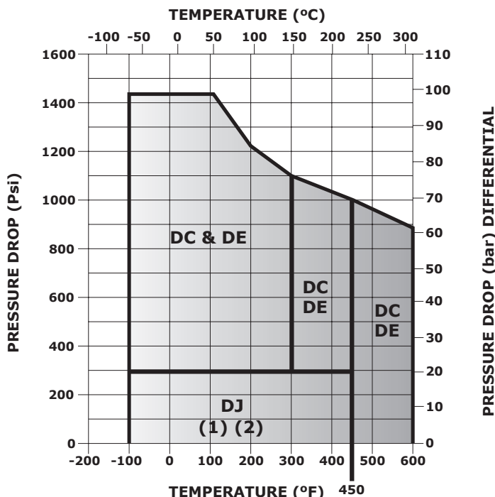
TRIM DC, DE, DJ, & DN - METAL SEATING WITH ASME CLASS 600 CF8M BODY
