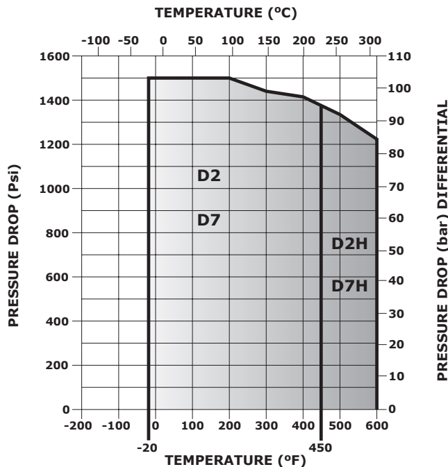
TRIM D2, D7, D2H, & D7H - FOR METAL SEATING WITH ASME CLASS 600 WCC OR WC9 BODY
